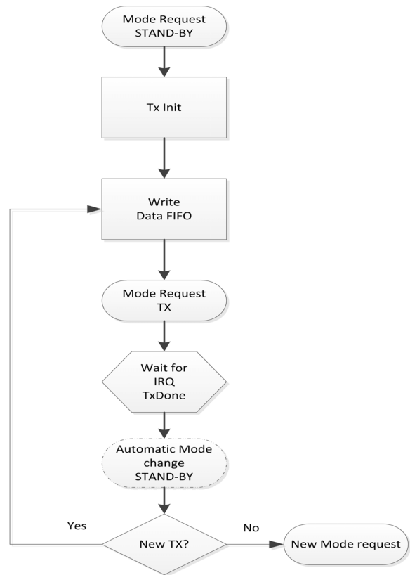
Figure 10. LoRa™ modulation transmission sequence.
