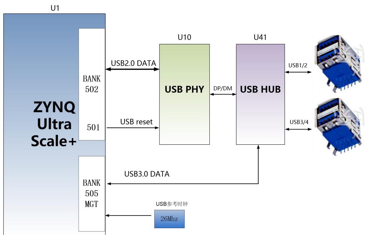
Figure 8-1: USB 3.0 Schematic
