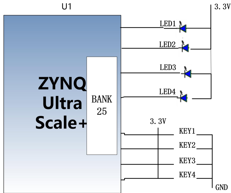
Figure 17-1: LED Schematic
