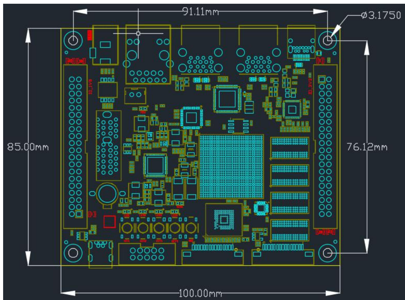
Figure 21-1: Size Dimension (Top View)
