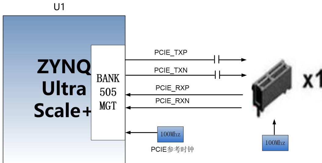
Figure 12-1: PCIe Schematic
