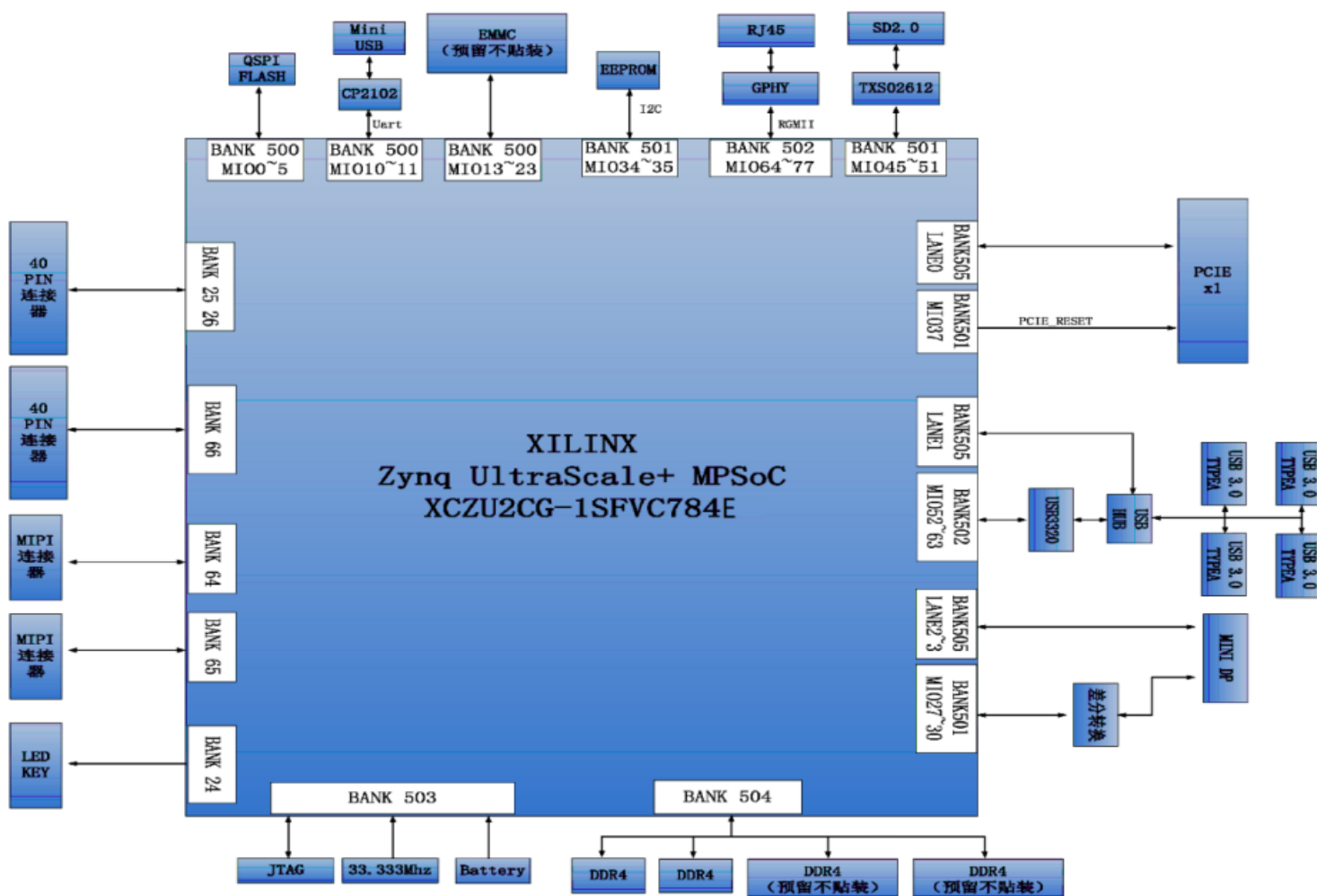
Figure 1-1: Board Schematic
