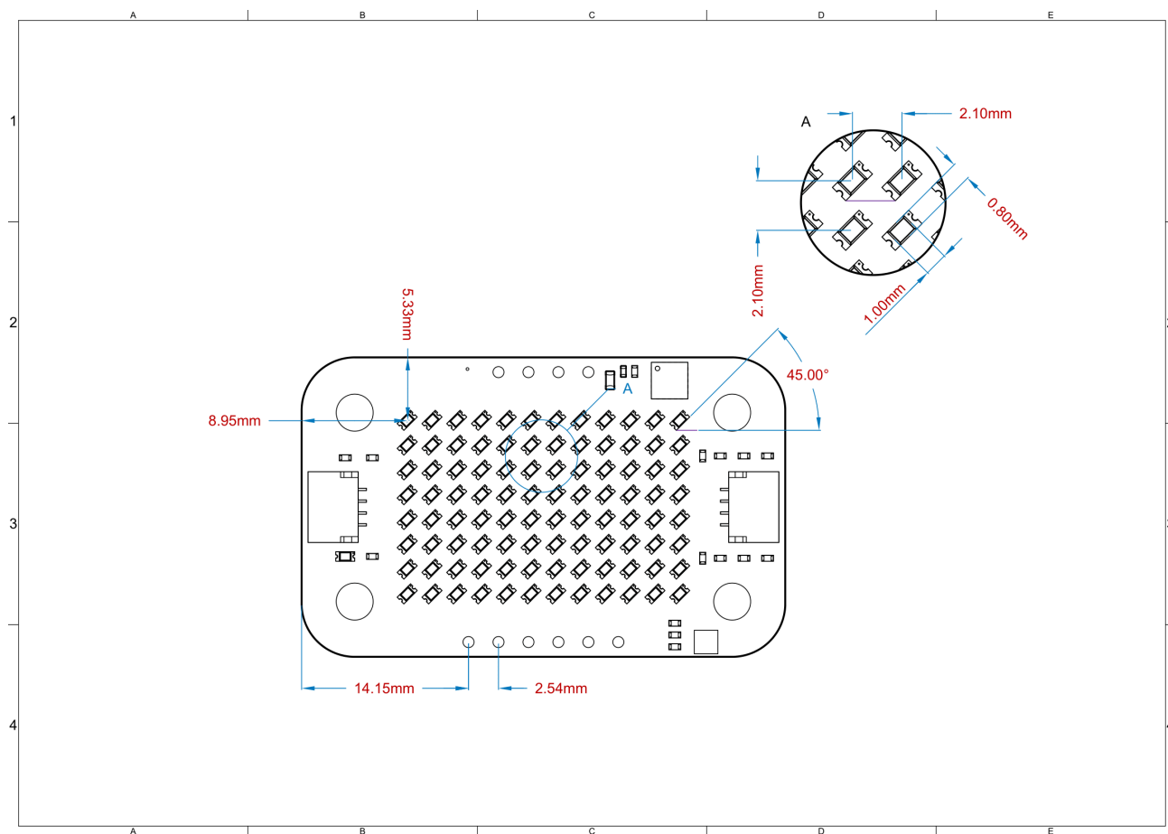
Modulino LED Matrix Mechanical Information
